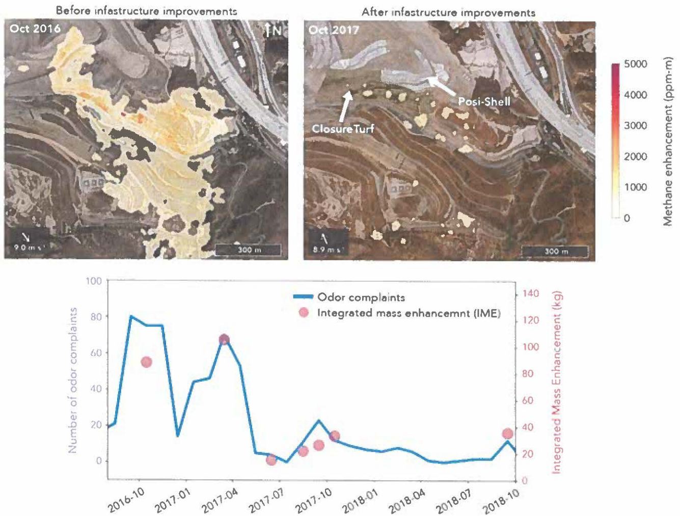
Figure 2. Reduction in methane emissions over intermediate cover slopes at the Sunshine Canyon Landfill. The top left panel shows the methane retrieved by AVIRIS-NG during its October 2016 overpass. The top right panel shows the reduction in methane concentration by the time of the October 2017 AVIRIS-NG overpass, due to the installation of ClosureTurf, Posi-Shell, and vegetative cover on intermediate slopes. The bottom panel shows the trend in odor complaints and AVIRIS-NG IME estimates during the California Methane Survey. Methane IMEs were jointly reduced with odor complaints as landfill improvement measures were implemented.
